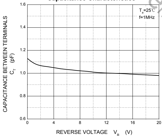
Capacitance Characteristics
